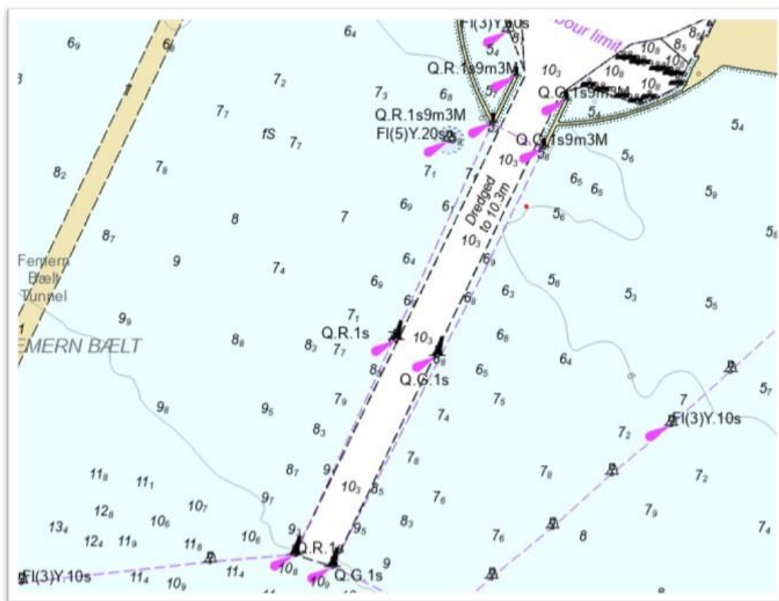
Figure 5: Position of access channel markers
