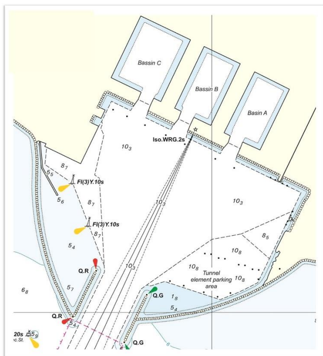
Figure 3: Water depths, breakwater lights and basin markers.
