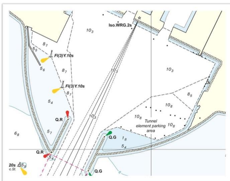
Figure 4 Position breakwater lights, basin markers and PEL
